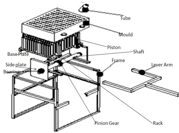
Figure 3. Exploded View of Chalk Moulding Machine.
